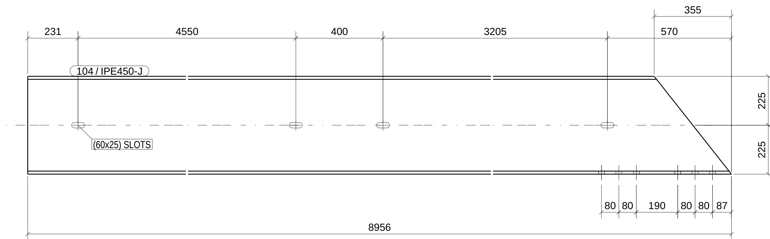
FRONT VIEW
